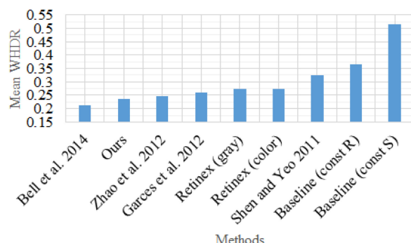
Fig. 13. The mean WHDR over all edges on the real image dataset. (This measure metric is biased to some extent as illustrated in Fig. 12. The reason that our approach lags behind the method in [17] has been further discussed in Section 4.2.)
