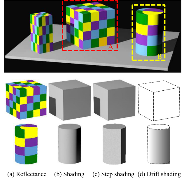
Fig. 4. Demonstration of our intrinsic image decomposition method on a simulated simple scene containing one cuboid, one cube, and one cylinder. Our method decomposes the input image into four images: (a) reflectance, (b) shading, (c) step shading, and (d) drift shading. The step-shading and drift-shading results are ideal decompositions according to our shading assumption. This is one of the main contributions of our approach.
