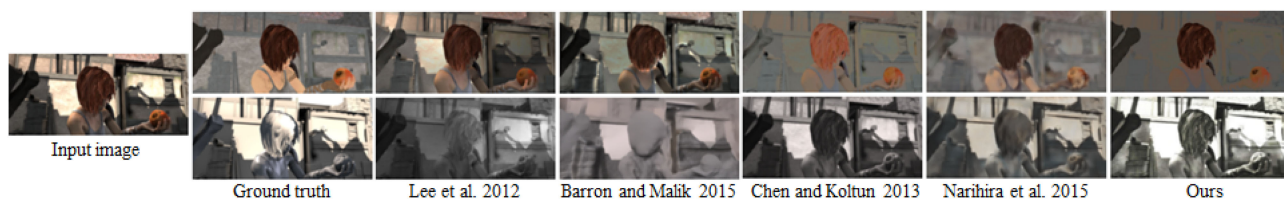
Fig. 17. Visual results of intrinsic image recovery on the MPI Sintel dataset. We compare the results of our approach with those by Lee et al. [19], Barron and Malik [14], Chen and Koltun [38], and Narihira et al. [22]. From the reflectance image by our method, we can clearly see that there is almost no shadow left, while large amount of remaining shadows exist in the other methods. Moreover, our shading image also has better visual sense than the others in that with the help of reinforcement process, it looks more natural and has higher resolution and articulation, as shown in the hair and the body part of the character.
