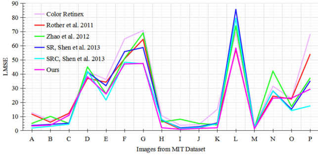
Fig. 10. Intuitive comparison between our method and other approaches on the MIT dataset. The y -axis label “LMSE” denotes “ \text{LMSE} \times 10^3 ”. (A) Box, (B) Cup1, (C) Cup2, (D) Deer, (E) Dinosaur, (F) Frog1, (G) Frog2, (H) Panther, (I) Paper1, (J) Paper2, (K) Raccoon, (L) Squirrel, (M) Sun, (N) Teabag1, (O) Teabag2, and (P) Turtle. We can see that our results have competitive performance, and outperform the others on most examples.
