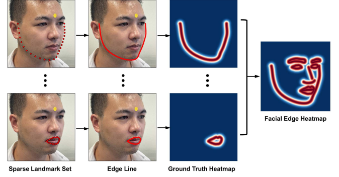
Fig. 6. An illustration of the ground-truth facial boundary heatmap generation process, where the standard deviation \sigma is set as 7. Each row represents the process of one specific facial boundary, including outer facial contour, outer/inner mouth, left/right eyebrow, upper/lower eyelid, and nose bridge/base.
