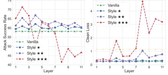
Figure 6. Study how synthesized style features affect the clean loss, which in turn impacts the attack success rate. The number of stars indicates the degree of change in original style features.
