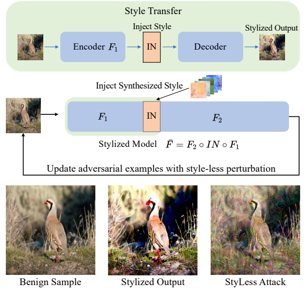
Figure 1. An overview of our StyLess attack. We create stylized model \bar{F} by injecting synthesized style features into the surrogate model ( F = F_2 \circ F_1 ) using an adaptive IN layer. StyLess reduces the use of non-robust style features in the vanilla surrogate model F , ultimately improving attack transferability.
