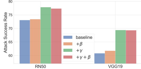
Figure 7. The effect of different statistics of style.
